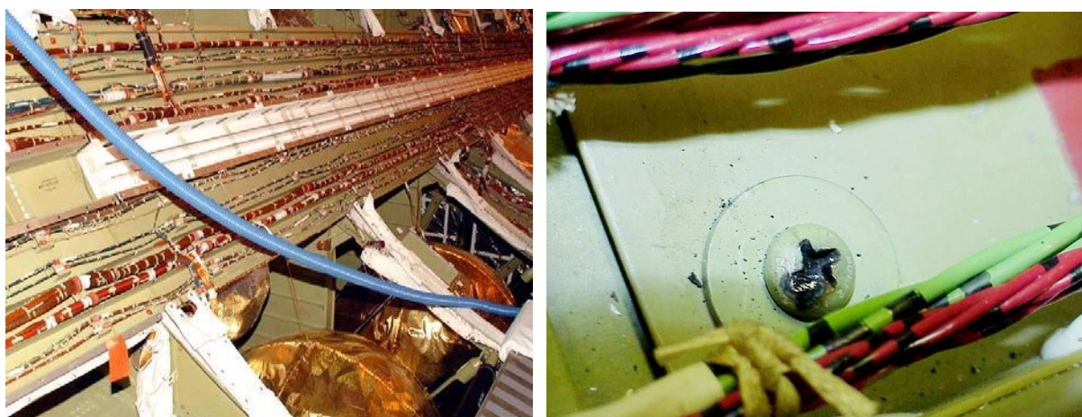
Figure 40. Orbiter Wiring in Payload Bay (left) and Typical Short-Circuit Source
