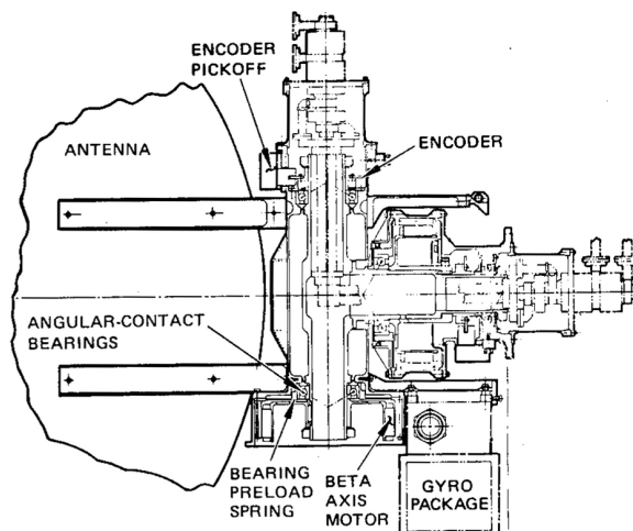
FIGURE 5. GIMBAL ASSEMBLY CROSS SECTION
